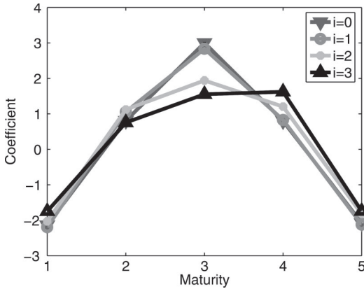
FIGURE 3. COEFFICIENTS IN REGRESSIONS OF AVERAGE (ACROSS MATURITY) EXCESS RETURNS ON LAGGED FORWARD RATES, \bar{r}x_{t+1} = \gamma^\top \mathbf{f}_{t-i/12} + \varepsilon_{t+1}
